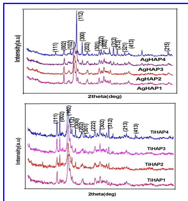
Fig. 1: XRD Spectra for Silver and Titanium doped HAP
